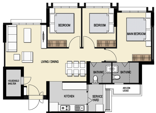
LAYOUT IDEAS FOR 4-ROOM
